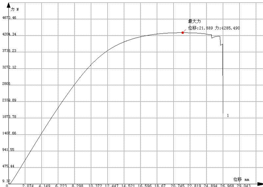
Force-displacement curve
