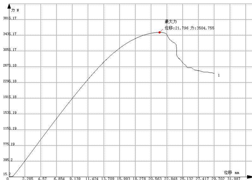
Force-displacement curve
