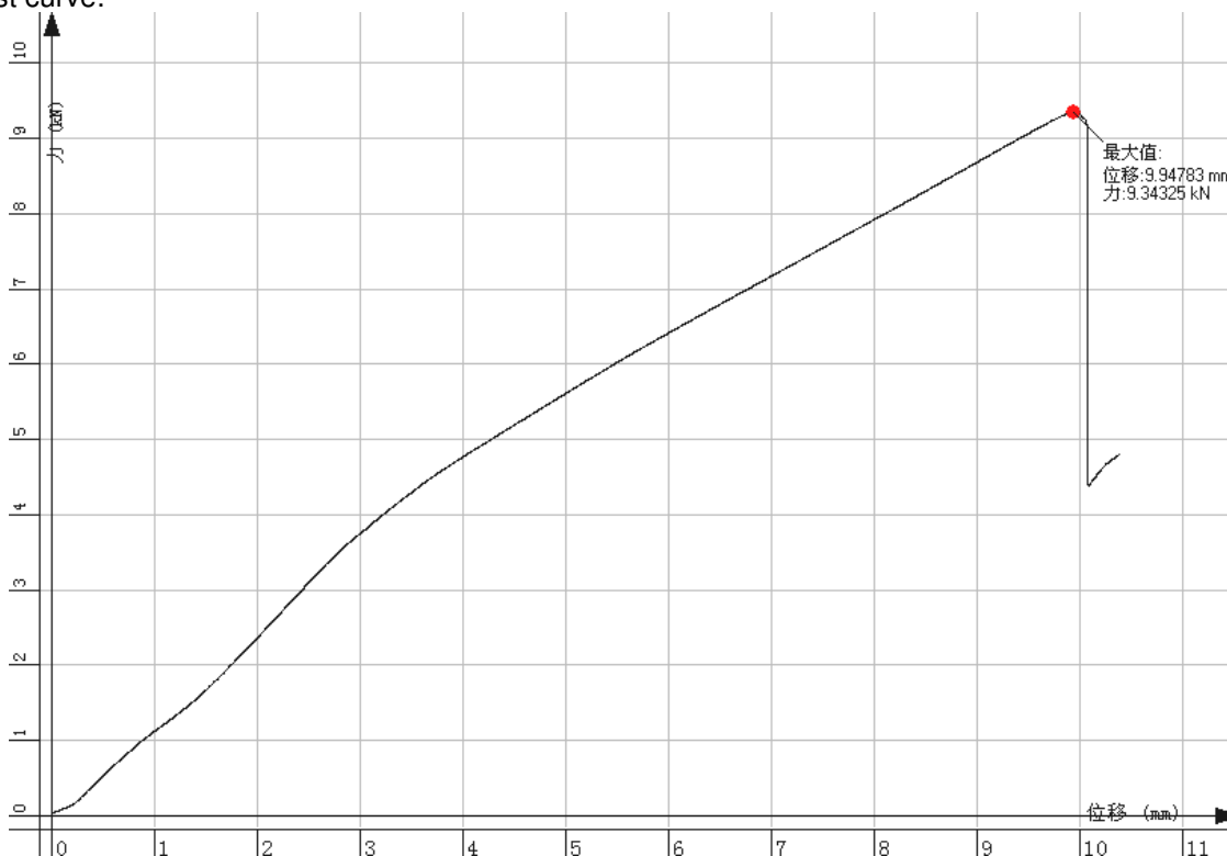
Force-displacement curve
