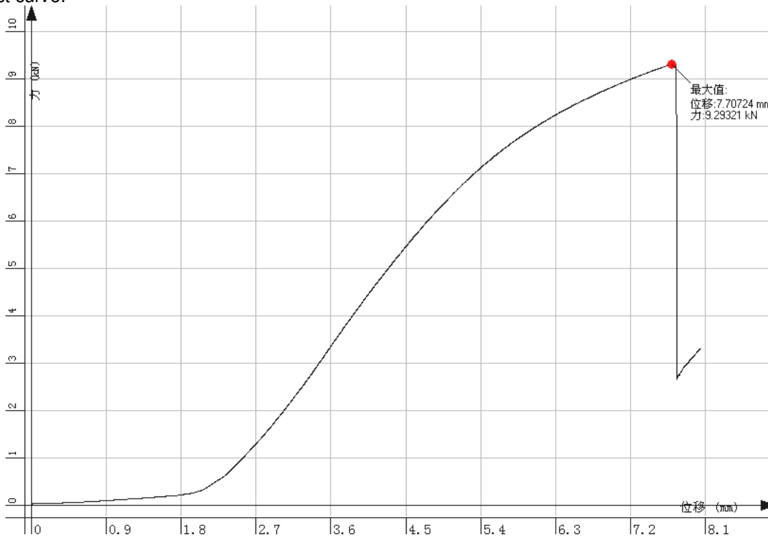
Force-displacement curve
