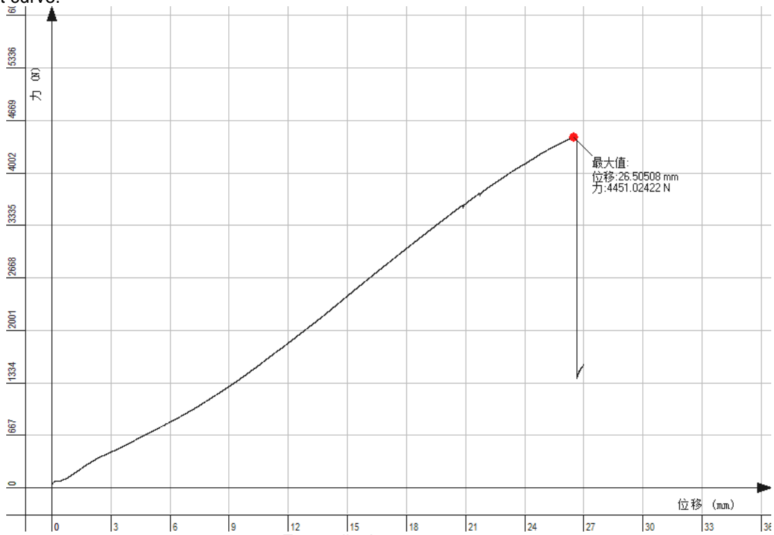
Force-displacement curve
