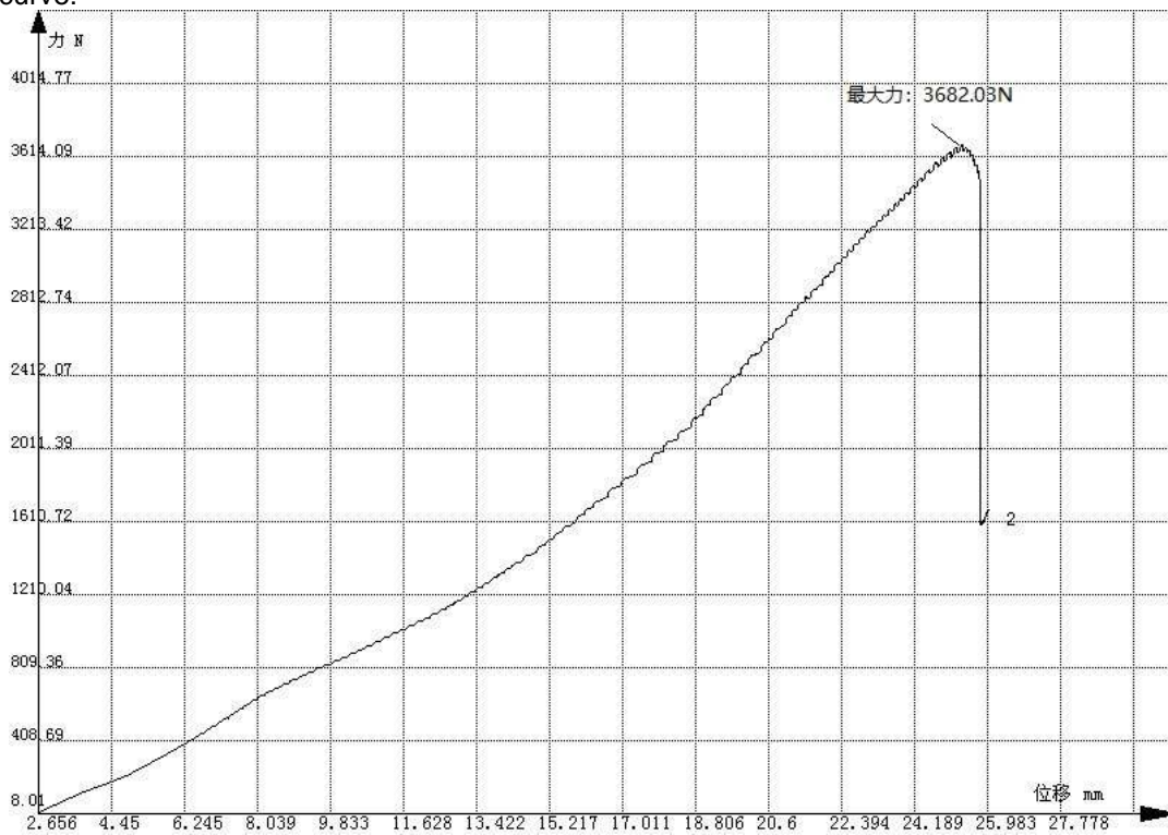
Force-displacement curve
